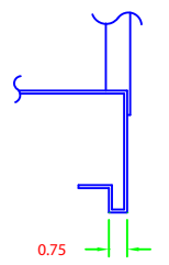
TYPICAL BASE DETAIL
